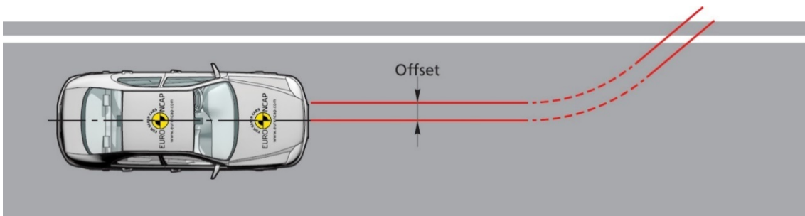
Figure 2: Lateral Path Error
