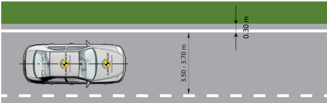
Figure 4: Layout of the lane markings
